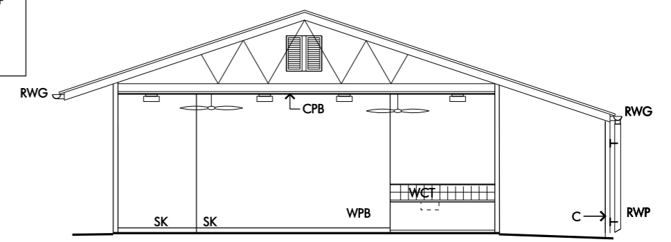
01 SECTION 1
